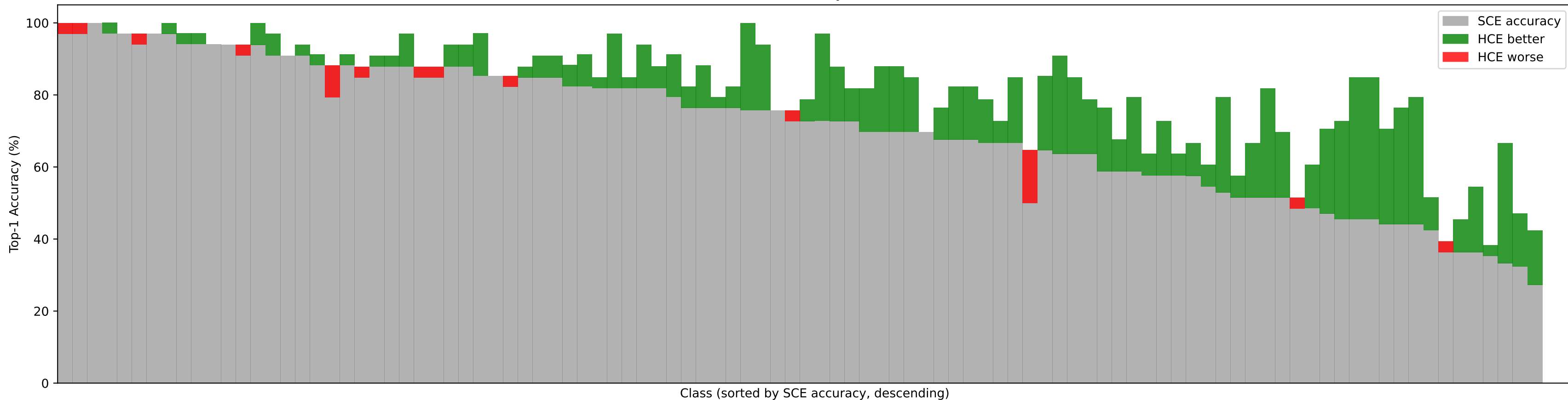
ResNet-50 — Per-leaf-class accuracy: SCE vs HCE (FGVC Aircraft)
